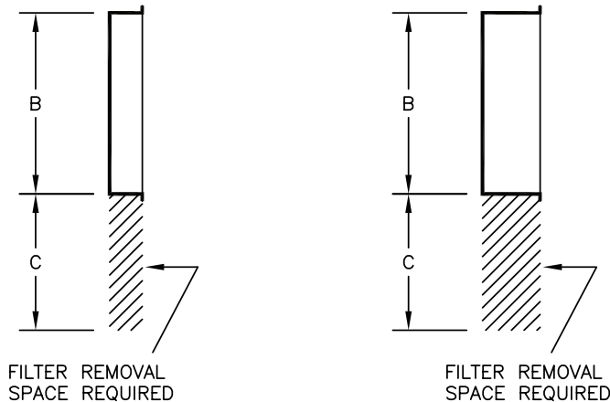
TOP VIEWS
