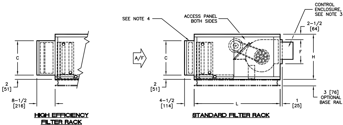
SIDE VIEWS
