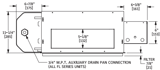
Model VLC Concealed Dimensional Data
